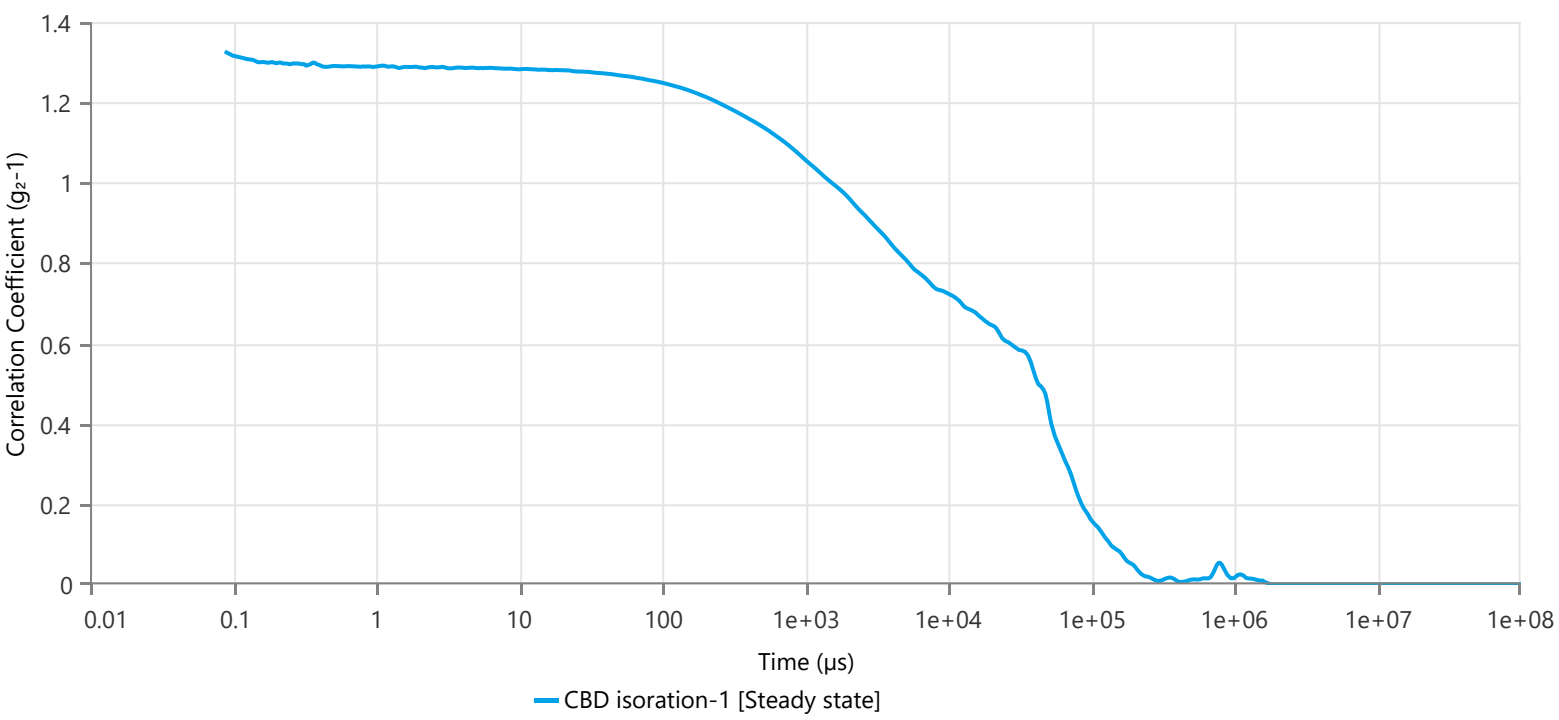
Correlogram
